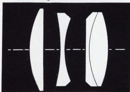
Agfa Color-Solinar 1:2,8/50 mm
